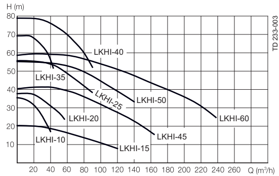
Volumetric flow
